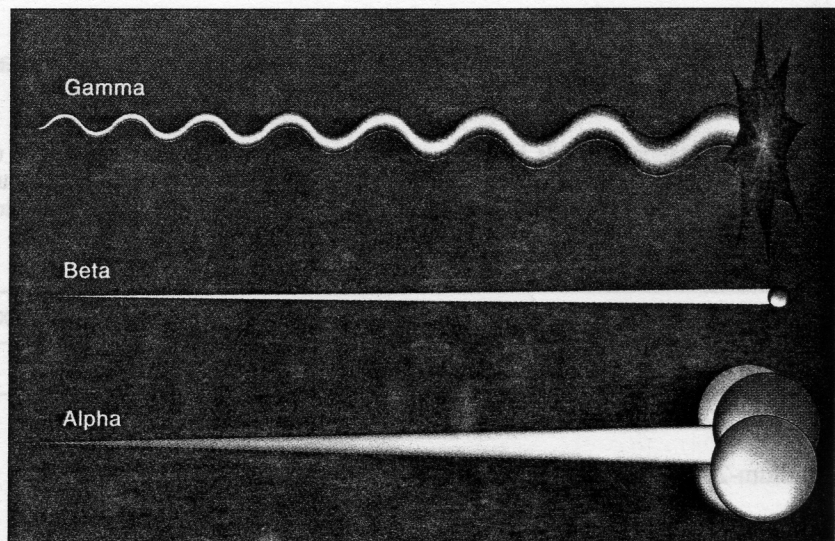
The three main types of radiation are gamma, beta, and alpha. Most damaging radiation in natural environments is caused by alpha radiation. Beta and gamma radiation generally are not a concern.
