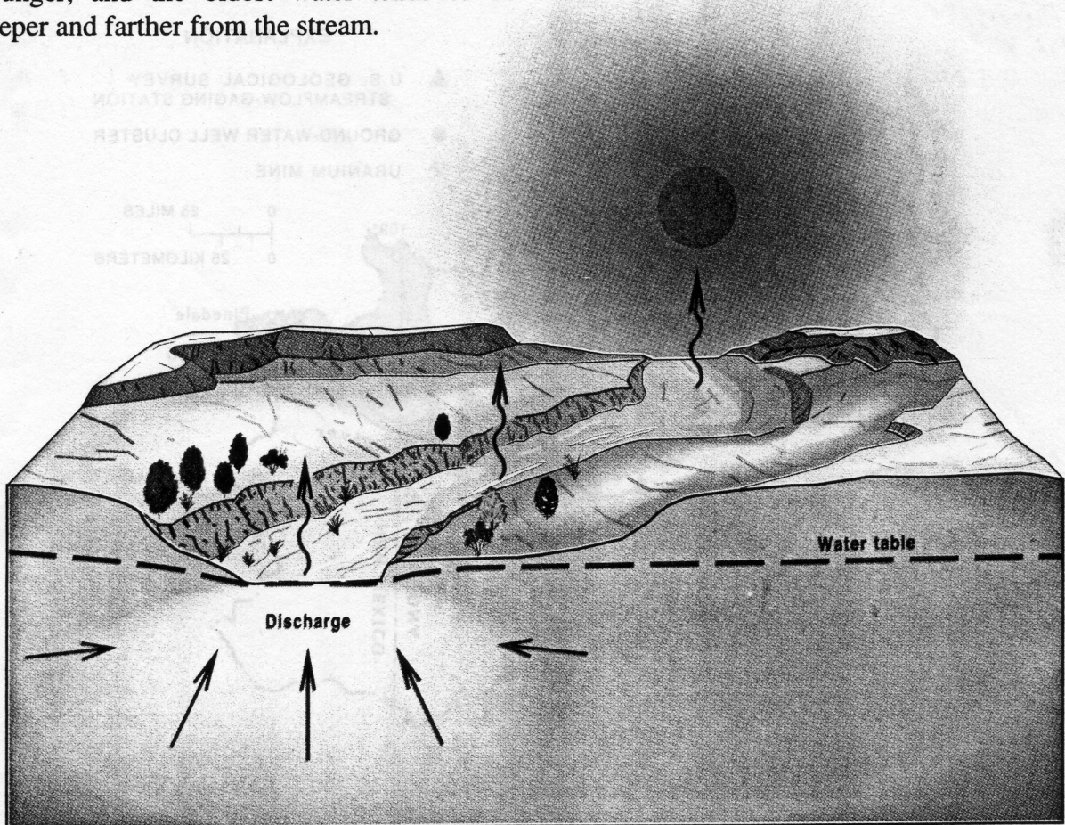
When the river is dry, ground water moves upward and is lost by evaporation through plants and sediments.
