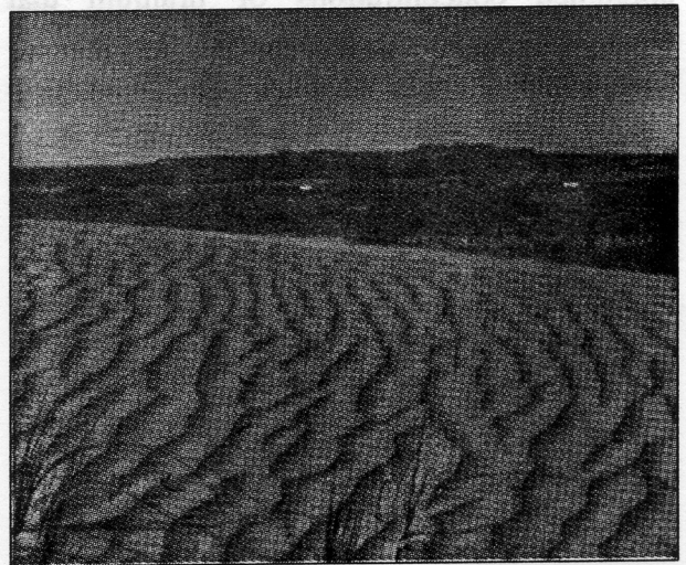
Radioactive substances on sediment may be transported in floods or carried as wind-borne particles. Breathing dust would not pose a health hazard unless continually inhaled over many years.
